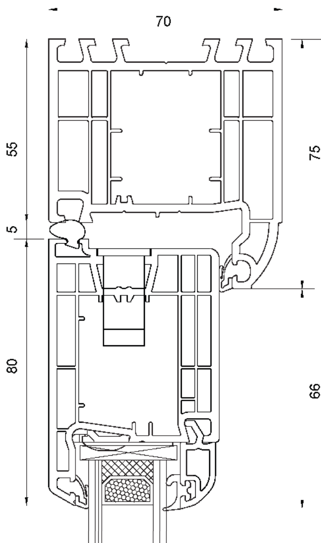
Head & and Side Section Detail
